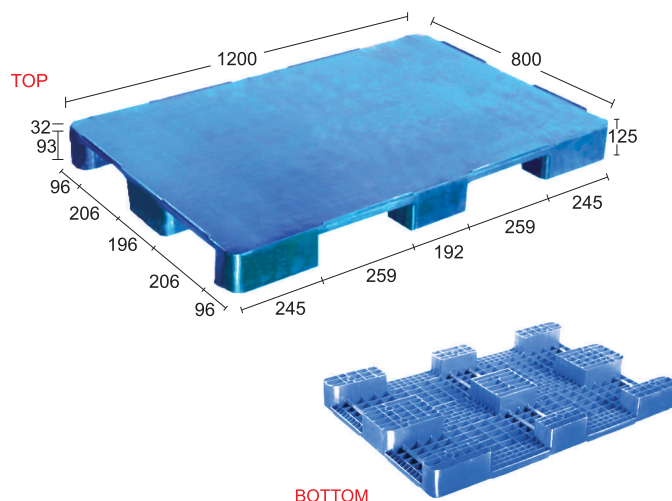
Model: SIM1280125 CDSS 9L (Supreme Injection Moulded Close Deck Single Side 9 Legs)
