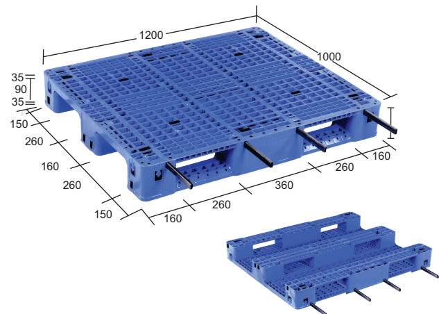
Model: SIM121016 AR PDSS 4 SRWS (MW) (Supreme Injection Moulded Arrow Perforated Deck Single Side 4 Steel Reinforced Width Side, Medium Weight)
