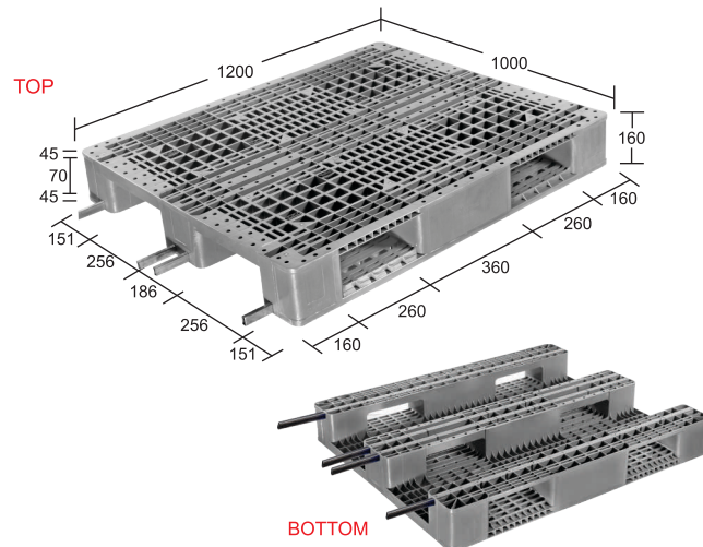
Model: SIM121016 PDSS SR (Supreme Injection Moulded Steel Reinforced Perforated Deck Single Side)
