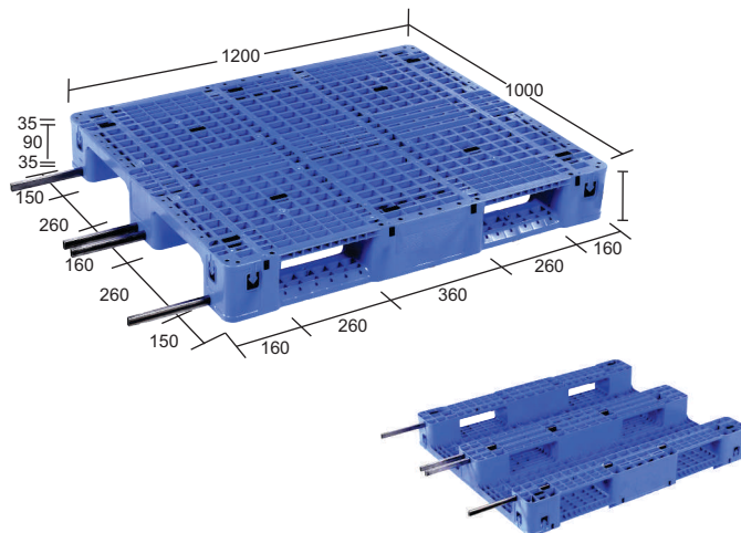
Model: SIM121016 AR PDSS 4 SR LS (MW) (Supreme Injection Moulded Arrow Perforated Deck Single Side 4 Steel Reinforced Length Side, Medium Weight)
