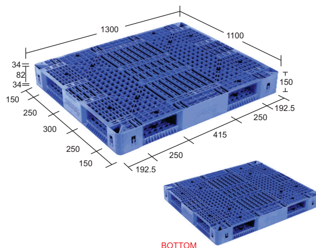
Model: SIM131115 PDD (Reversible) (Supreme Injection Moulded Perforated Double Deck)
