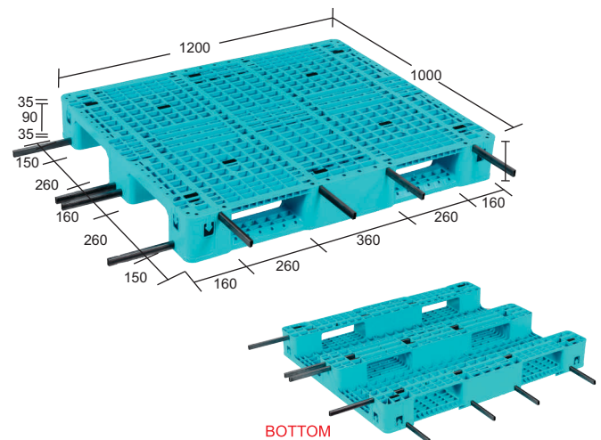
Model: SIM121016 AR PDSS 8 SR (Supreme Injection Moulded Arrow Perforated Deck 8 Steel Reinforced Single Side)
