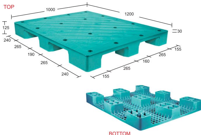
Model: SIM1210125 CDSS 9L (Supreme Injection Moulded Close Deck Single Side 9 Legs)
