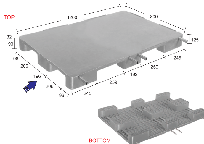
Model: SIM1280125 CDSS SR 9L (Supreme Injection Moulded Steel Reinforced Close Deck Single Side 9 Legs)
